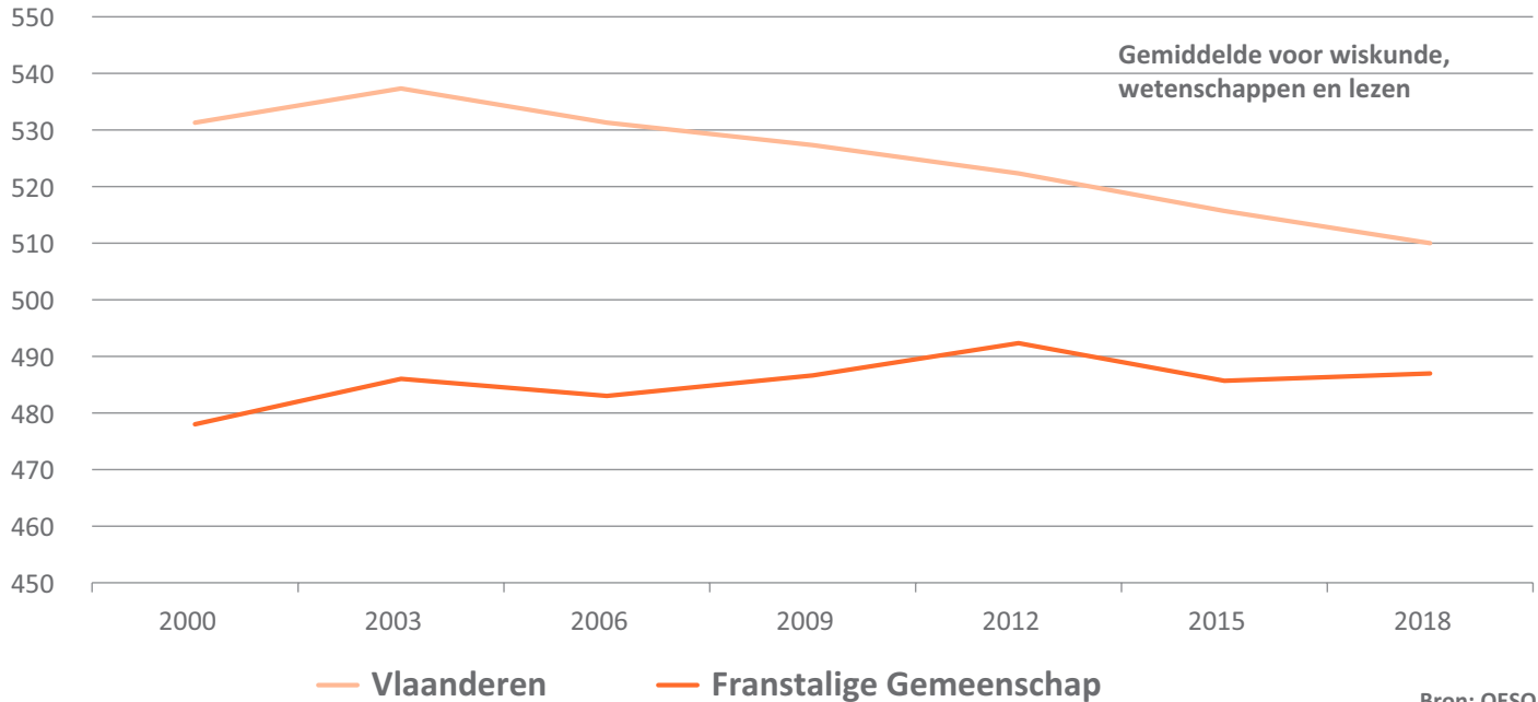
PISA-scores
